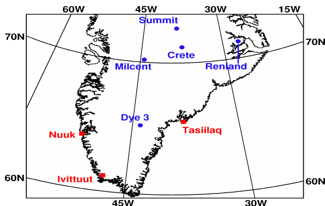
Figure 1. Location of the Greenland ice core drill sites (blue) and temperature stations (red) used for this survey.
