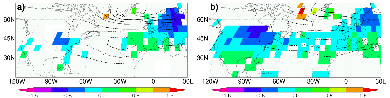
Figure 2. The spatial response of surface pressure (contours in hPa) and temperature (scale in ^{\circ}\text{C} ) corresponding to a 1\sigma increase in the ice core PC1 time series. (a) is based on a linear regression of the PC1 time series versus CRU Dec-Mar surface pressure and temperature data for 1874-1970 and 1857-1970 (year of Jan) respectively. (b) as for (a) but only for Dec-Mar 1897-1926 (see text for details). Grid points with more than 10% missing temperature data are left blank.
