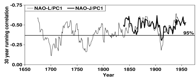
Figure 3. Running 30 year Pearson correlations between the ice core PC1 time series and December to March means of the NAO-L and NAO-J indices. Correlations numerically larger than 0.36 are significant at the 95% level.
